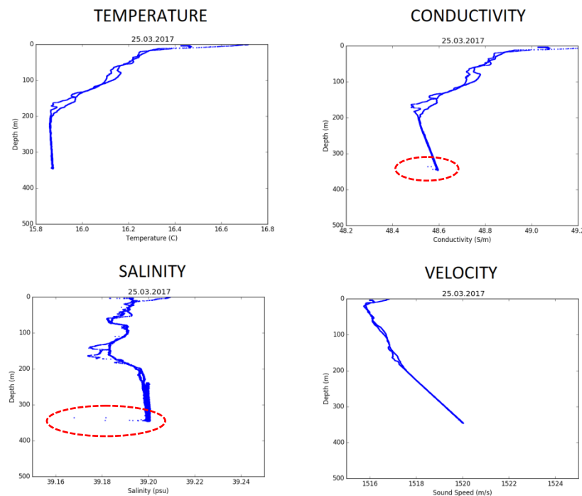
Figure 2. Temperature, Conductivity, Salinity and Sound Velocity profiles according to the 25-3-2017 survey in the North Basin of Santorini. Anomalies in the profiles are circled with dashed ovals.
